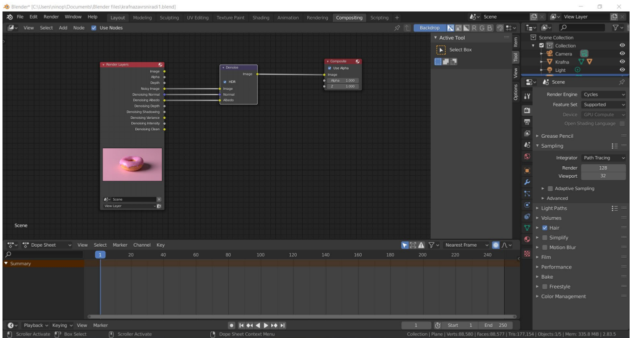
Slika 28: Compositing view
